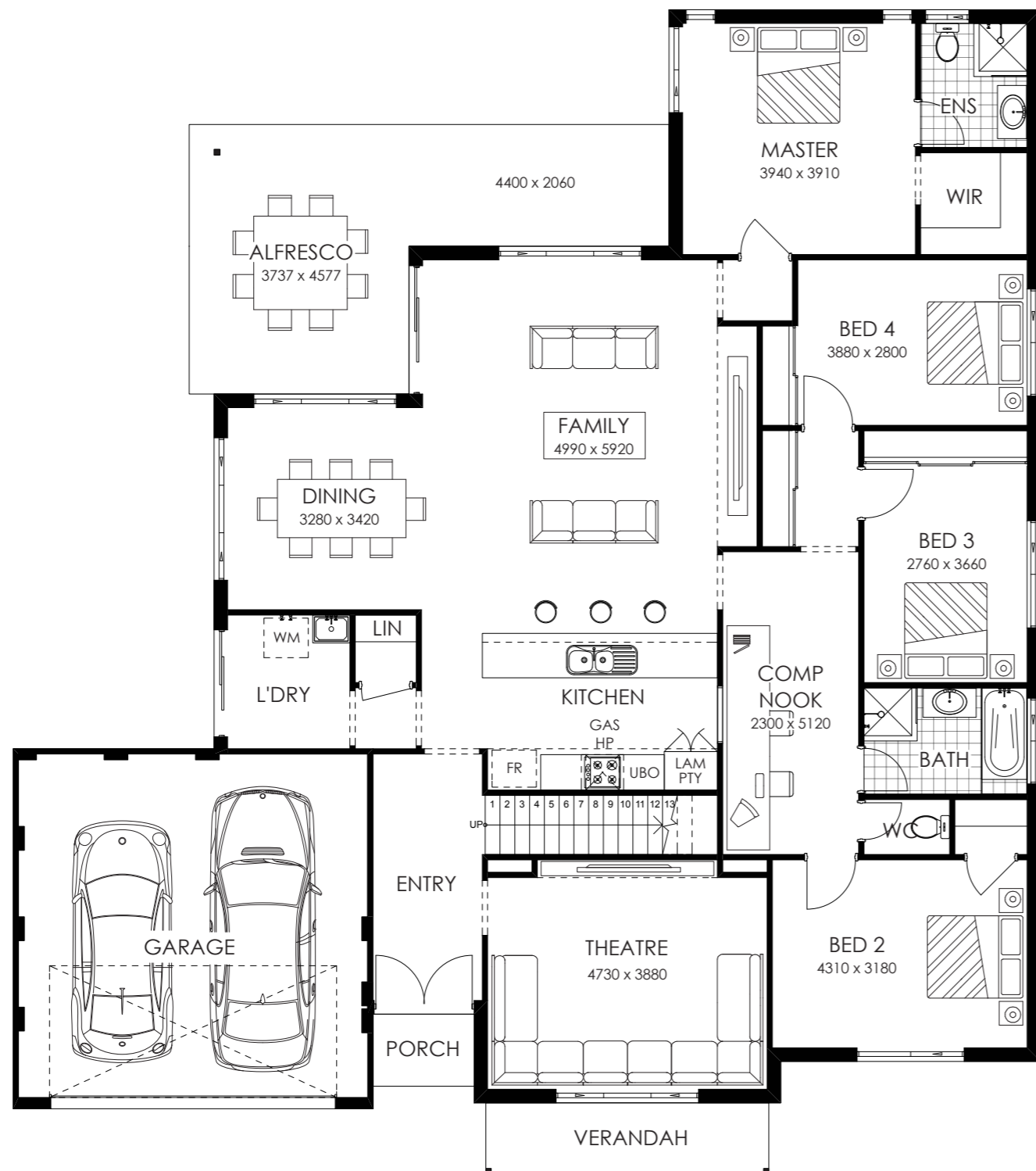
FLOOR PLAN
