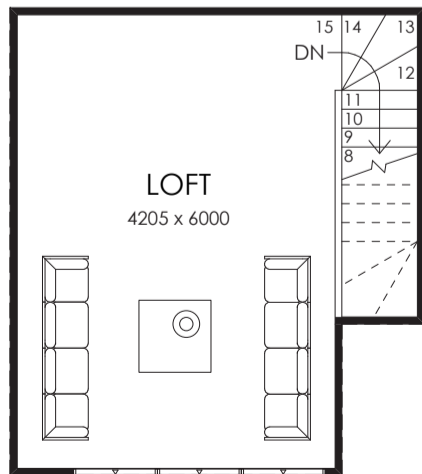
LOFT FLOOR PLAN 1:100
