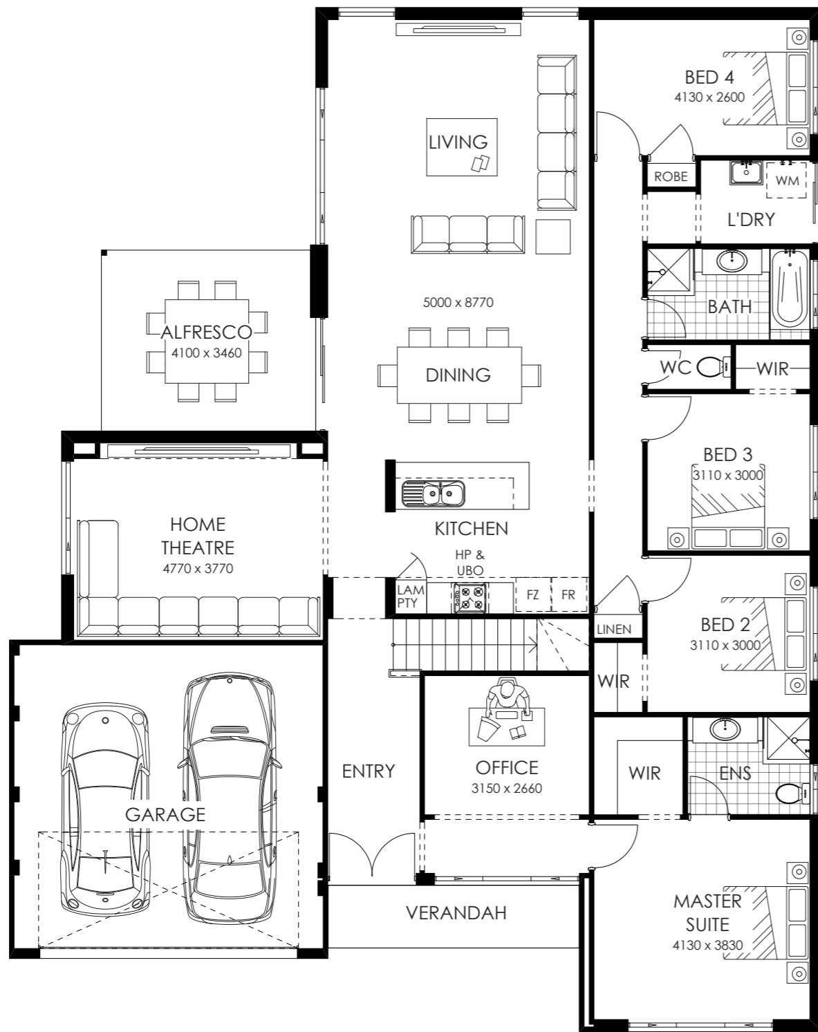
FLOOR PLAN
